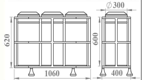
CK-8001 Profile Stand Recycle 3-Bins, Stainless Steel
