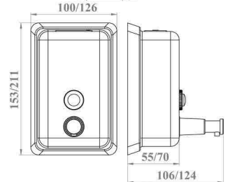
SB-5520 Wall Mounted Soap Dispenser, AISI 304 Stainless Steel, 500/1000ml
