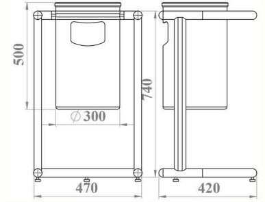
CK-2106 Outdoor Wastebin 35 LT
