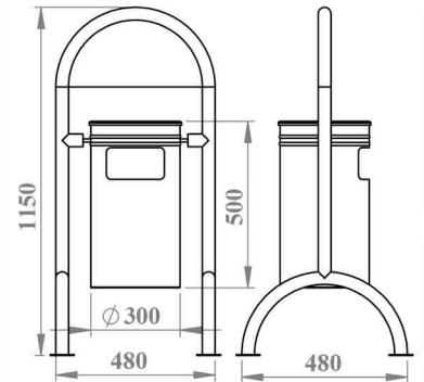
CK-2107 Outdoor Wastebin 35 LT
